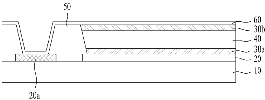
FIG.1 RELATED ART
